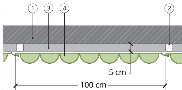
HORIZONTAL DETAILED SECTION
